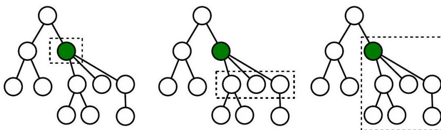
Fig. 13.10: Scope in LDAP searches. The filled circle is the chosen base object.
