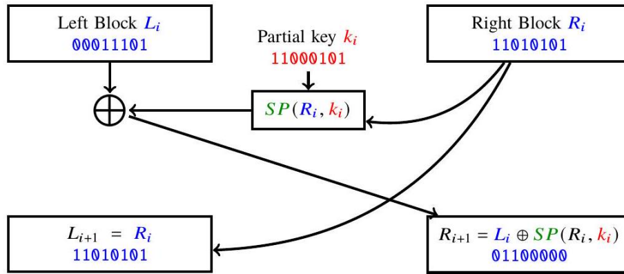
Fig. 7.6: Operation of a stage in a Feistel network
