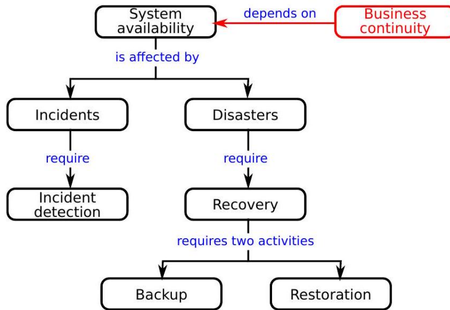
Fig. 14.2: BCP concepts
